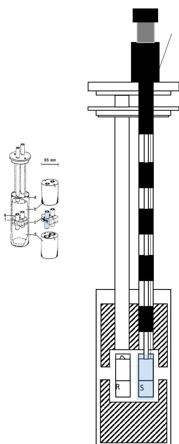
Calorimetric Channel
